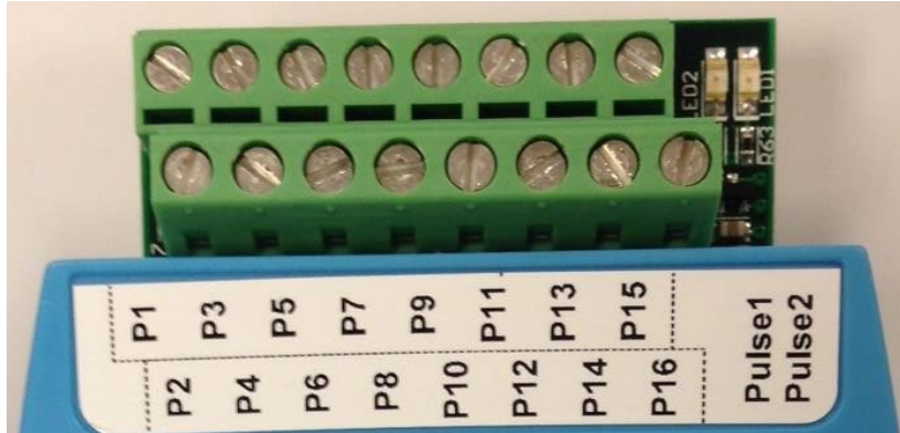
Counting from Left to Right: P1 to P16 Lower Shelf is Odd Pins
